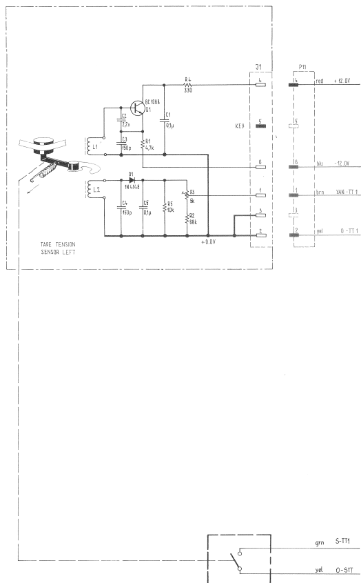
A6 Sensor board, left Abtasterprint, links Circuit analyseur, gauche 1.067.190
