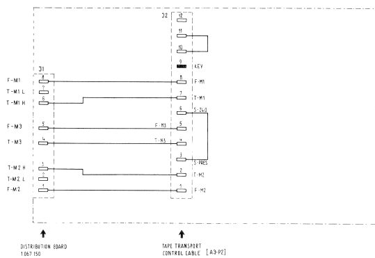
A5 TAPE TRANSPORT CONTROL 1.067.130
